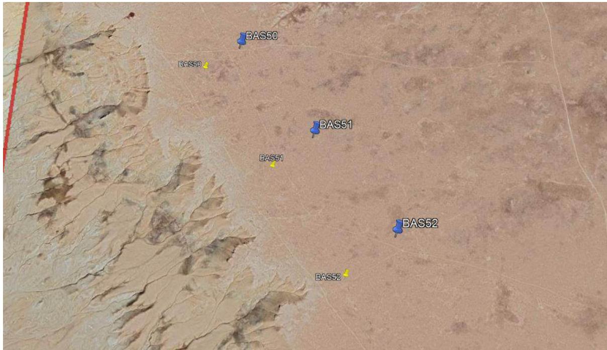
Figure 7-12 Three micrositied turbines maintaining 2km buffer from Lake Ayakagitma
