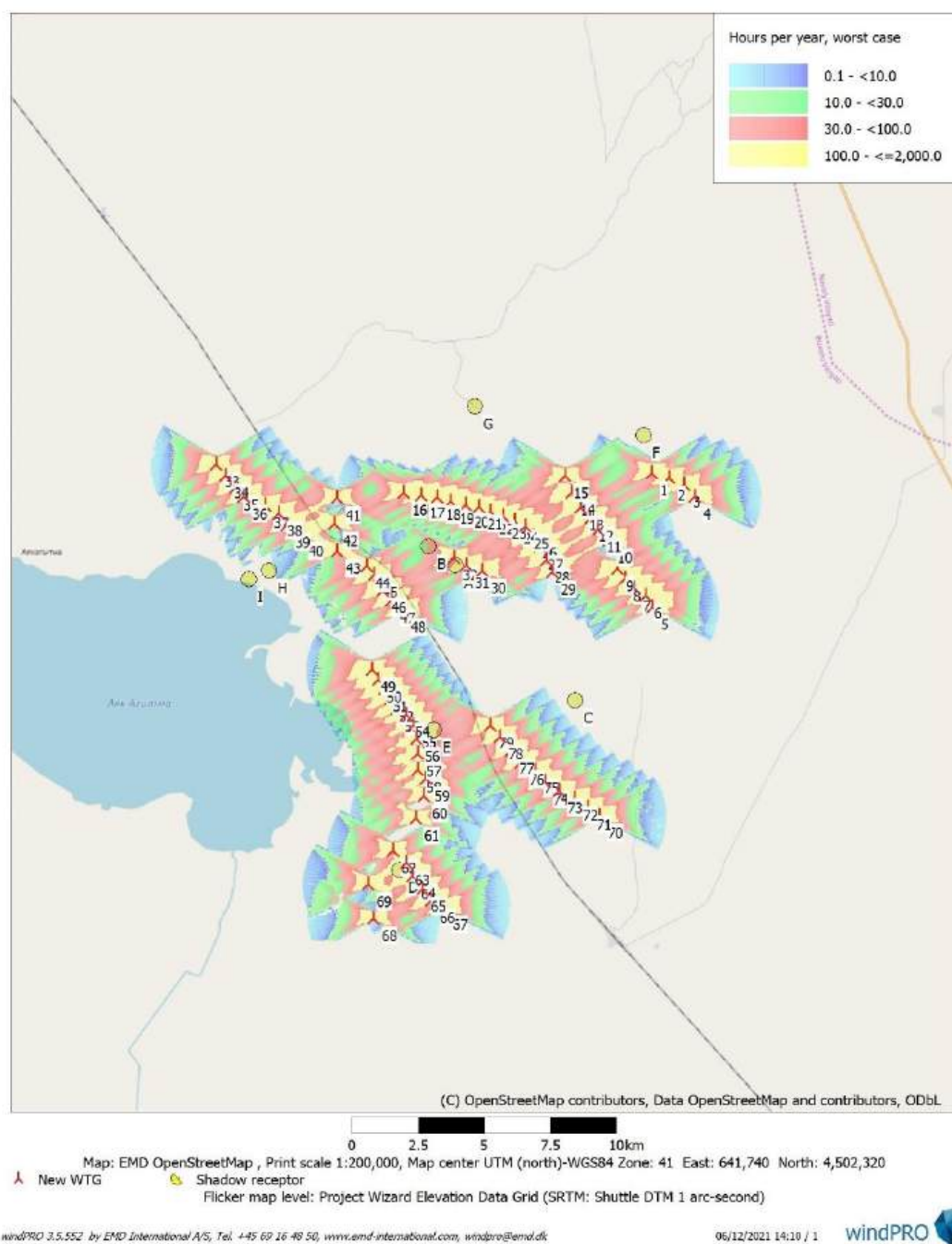
Figure 15-2 WBG/IFC Worst Case Shadow Hours Per Year
