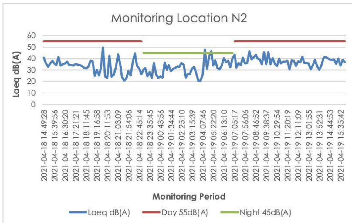
Figure 9-3 Noise Monitoring Result at N2
