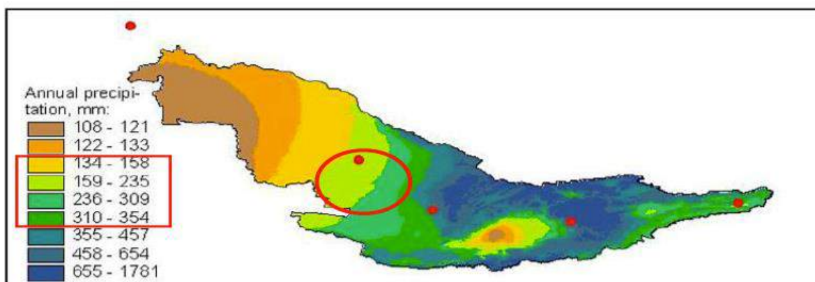
Figure 8-6 The average annual rainfall Values of the Bukhara Basin Between 2000 & 2020
