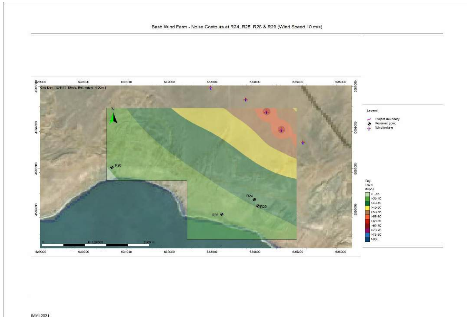
Figure 9-16 Noise Contour at the Project site R24, R25, R28, R29 (10m/s Wind Speed)
