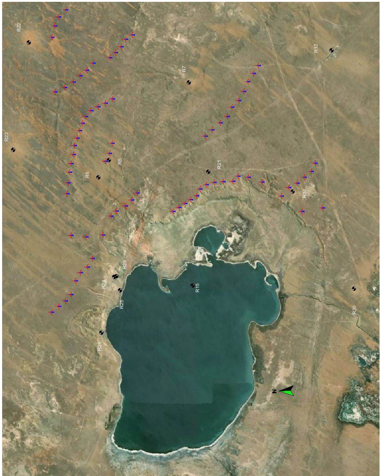
Figure 1 Bash Wind Farm Project, Turbine & Receptor Locations
